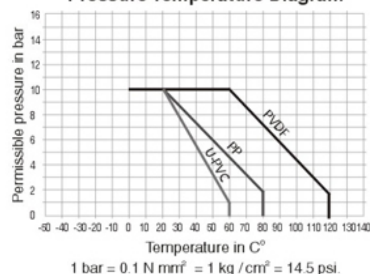
Pressure Temperature Diagram
